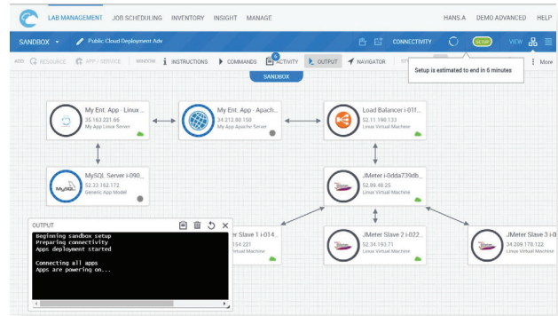
On-demand deployment of virtualized environments
